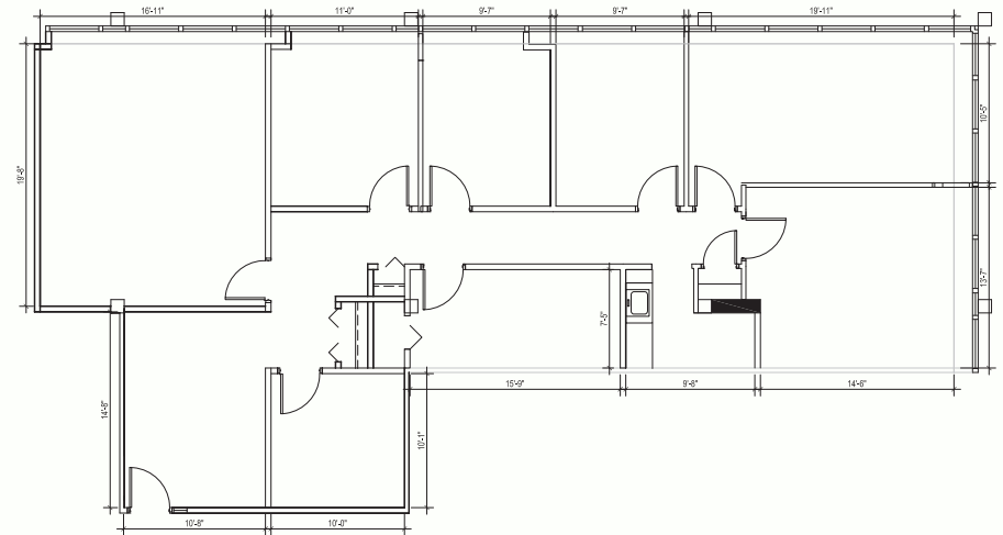
SUITE 310 - FLOOR PLAN sc: 1/8" = 1'-0"
