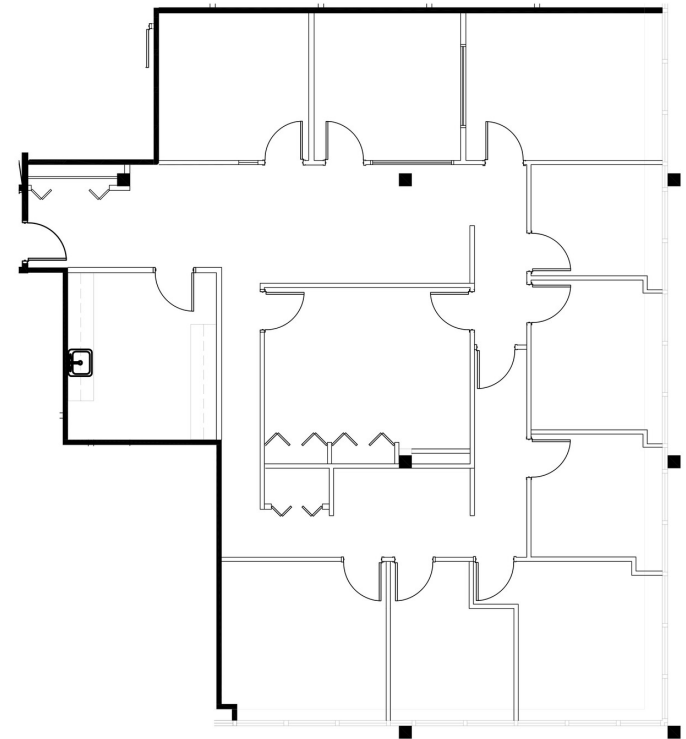
SUITE 230 - FLOOR PLAN sc: 1/8" = 1'-0"
