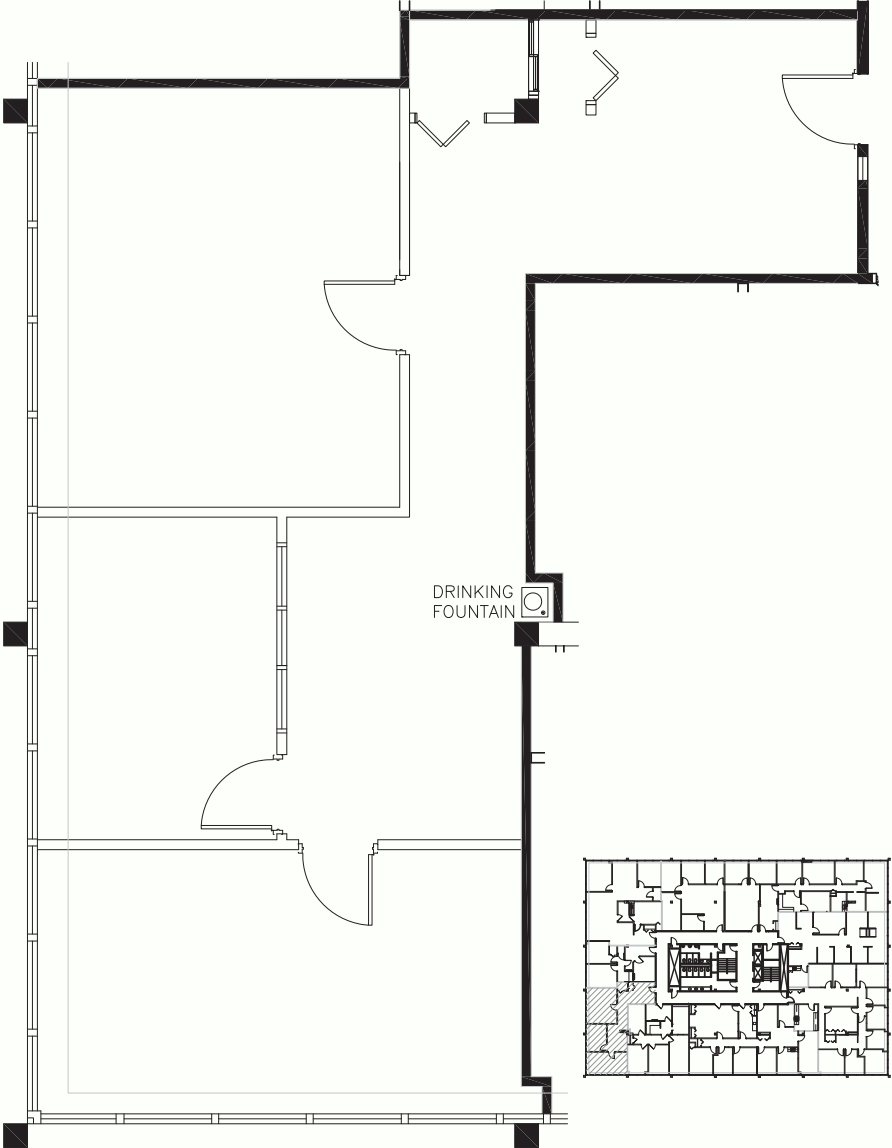
SUITE 208 - FLOOR PLAN sc: 3/16" = 1'-0"
